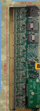
MMFE8 Readout Card
