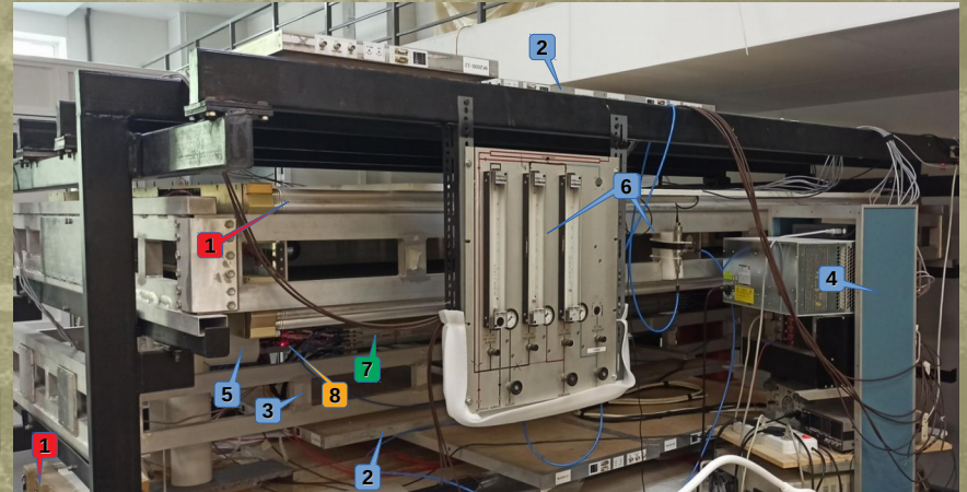
A general purpose Cosmic Test Stand in DLNP JINR
